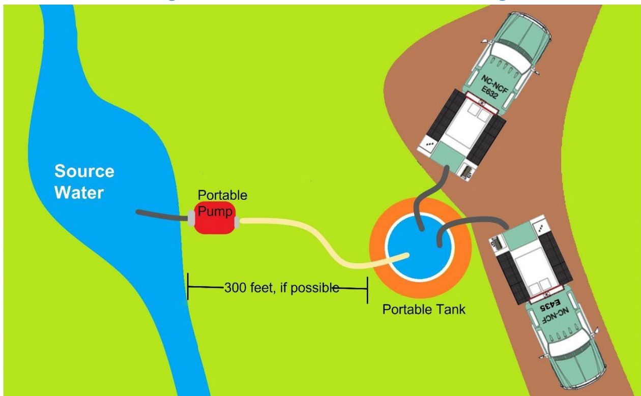
Figure 2: Engine + tender portable tank drafting
