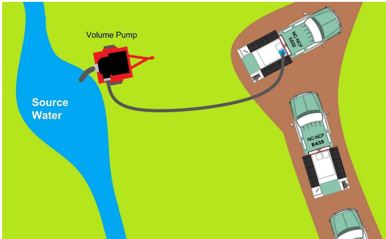
Figure 1: Preferred option for drafting - engine + tender top fill
